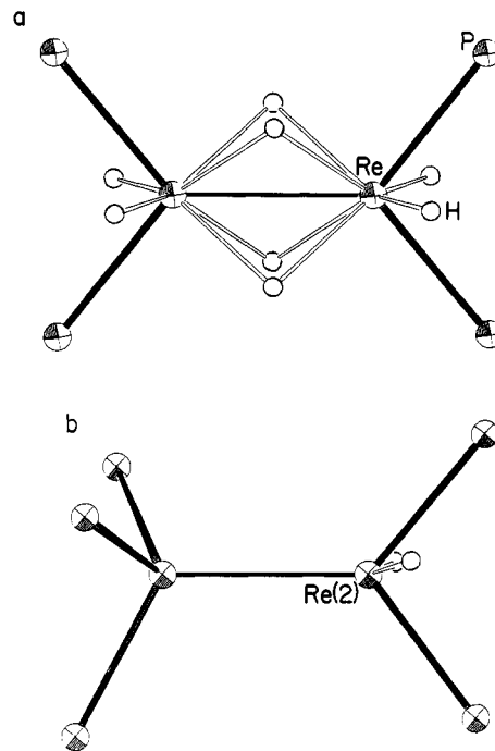
Figure 1. ORTEP drawings of the inner coordination spheres of (a) \text{H}_8\text{Re}_2(\text{PMe}_2\text{Ph})_4 4 and (b) \text{H}_6\text{Re}_2(\text{PMe}_2\text{Ph})_5 , oriented to show the structural relationship between the two. 16 Note that only two of the six metal-bound hydrogens have been located in \text{H}_6\text{Re}_2(\text{PMe}_2\text{Ph})_5 . These yield a terminal ligand environment about \text{Re}(2) which closely mimics that in \text{H}_8\text{Re}_2(\text{PMe}_2\text{Ph})_4 .
